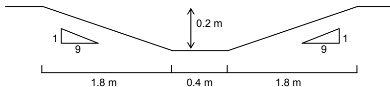
Figure 13.3-M: Swale Width and Side Slopes Cross Section
