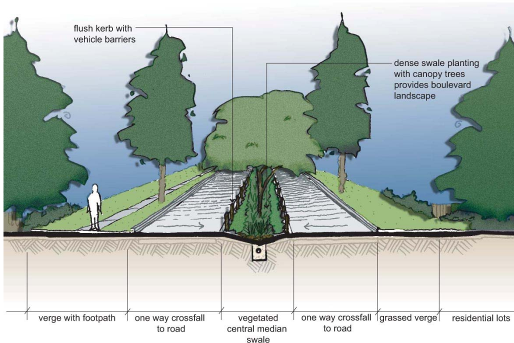
Figure 13.3-G: Landscape Treatment of a Vegetated Swale in Central Median
