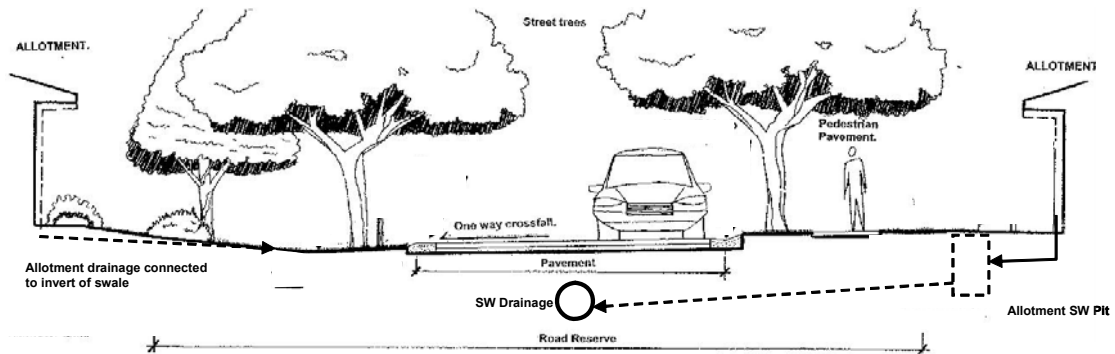
Figure 13.3-K: Conceptual Configuration of a Swale
