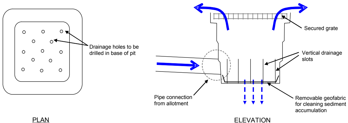
Figure 13.3-C: Example of surcharge pit for discharging concentrated runoff into a swale
