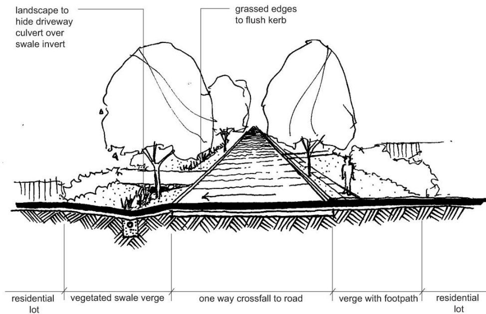
Figure 13.3-F: Landscape Treatment of Vegetated Swale on Single Side of Road
