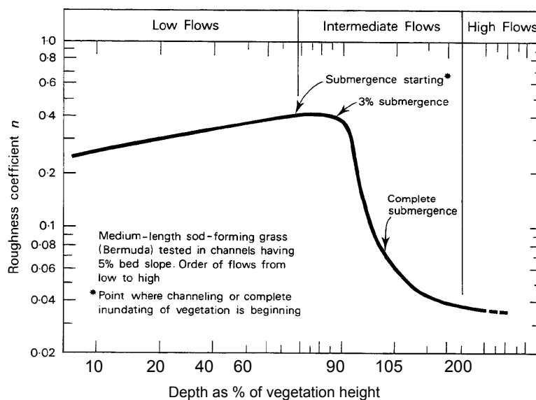
Figure 13.3-B: Impact of Flow Depth on Hydraulic Roughness
