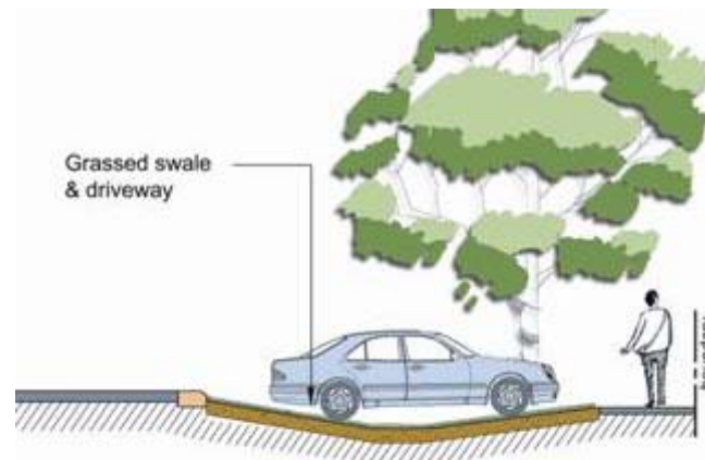
Figure 13.3-A: Typical arrangement of a swale 'at-grade' driveway crossing
