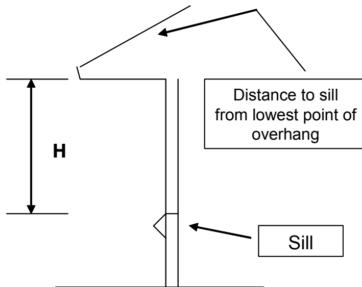
Figure 2: Schematic of overhangs and sills relevant to Table 1.
