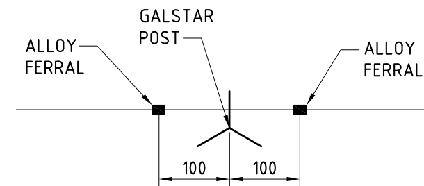
PLAN VIEW OF IN LINE BRAIDED WIRE FASTENING
