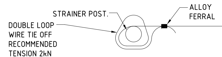
PLAN VIEW OF STRAINER POST BRAIDED WIRE FASTENING
