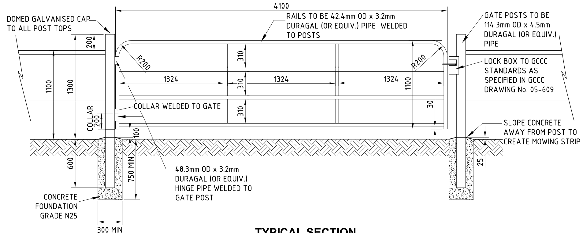
TYPICAL SECTION
