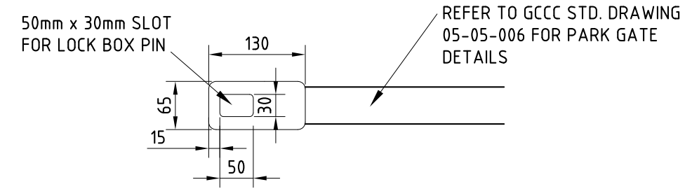
TONGUE TOP VIEW
