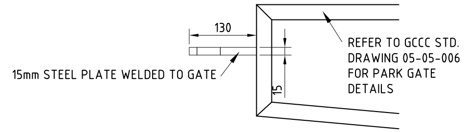
TONGUE SIDE ELEVATION
