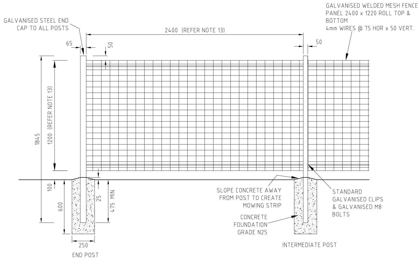
TYPICAL SECTION
