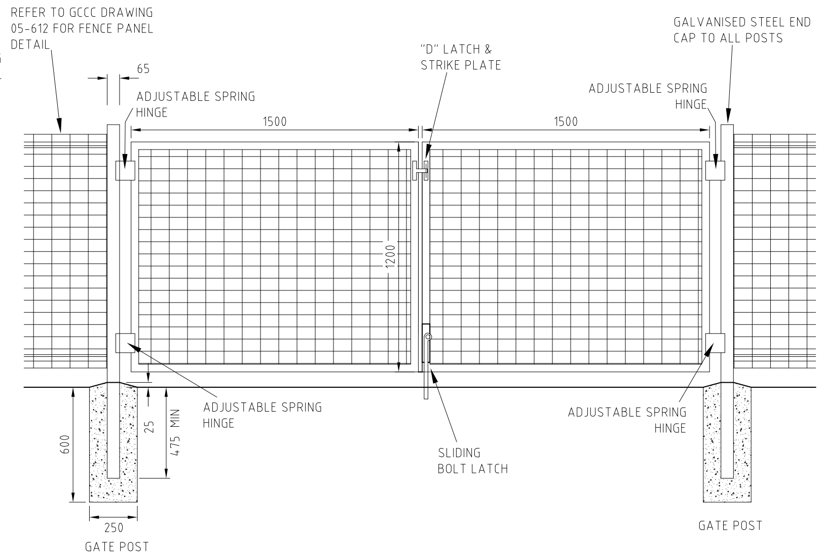
DOUBLE GATE
