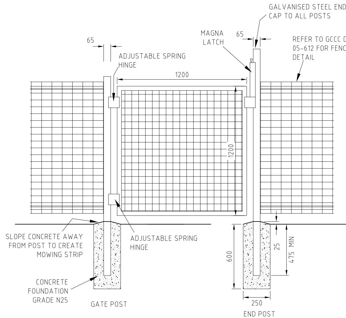
SINGLE GATE
