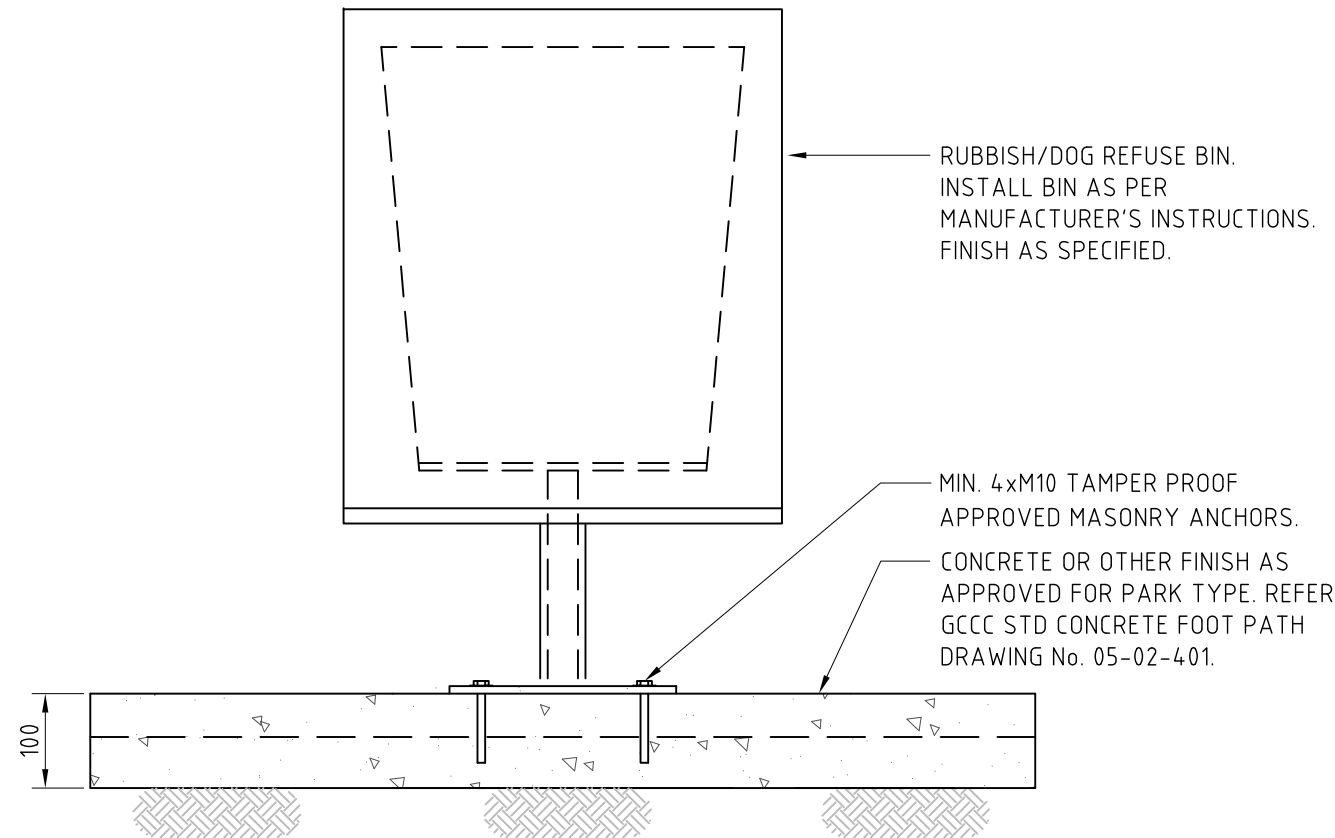
RUBBISH BIN IN CONCRETE PAVEMENT - SECTION
