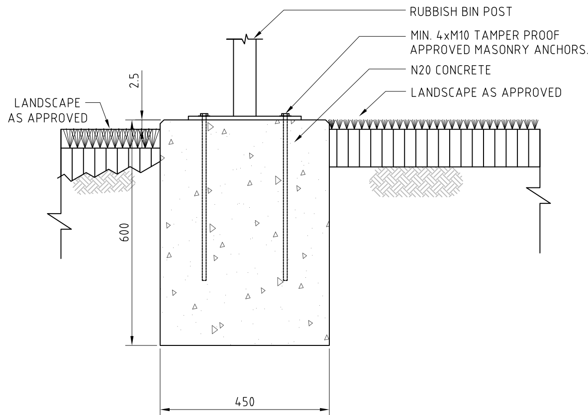
FOOTING IN TURF / GARDEN BED - SECTION
