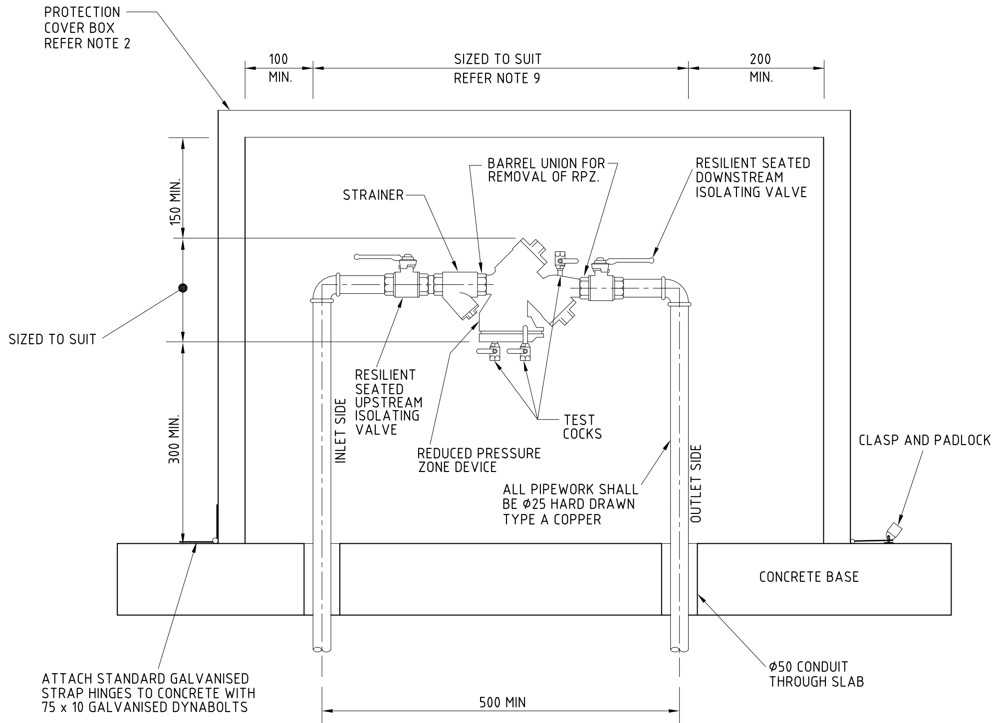
TYPICAL 25 Dia RPZ DEVICE INSTALLATION SEMI-DIAGRAMMATIC
