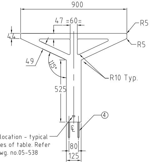
RIGHT VIEW
