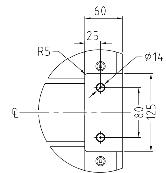
DETAIL D
