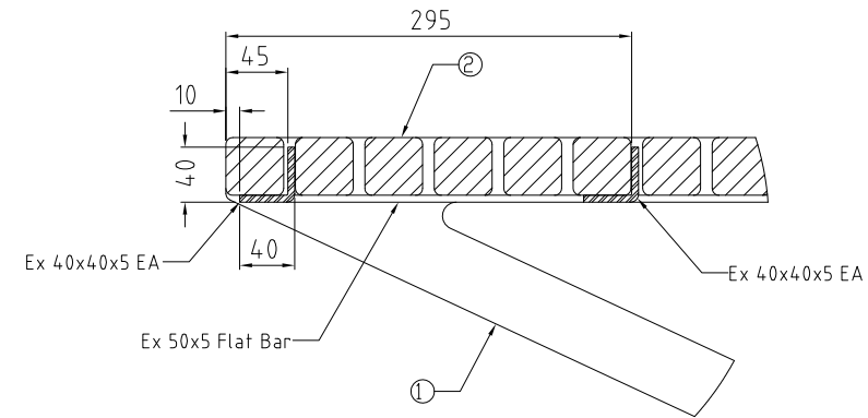
DETAIL C
