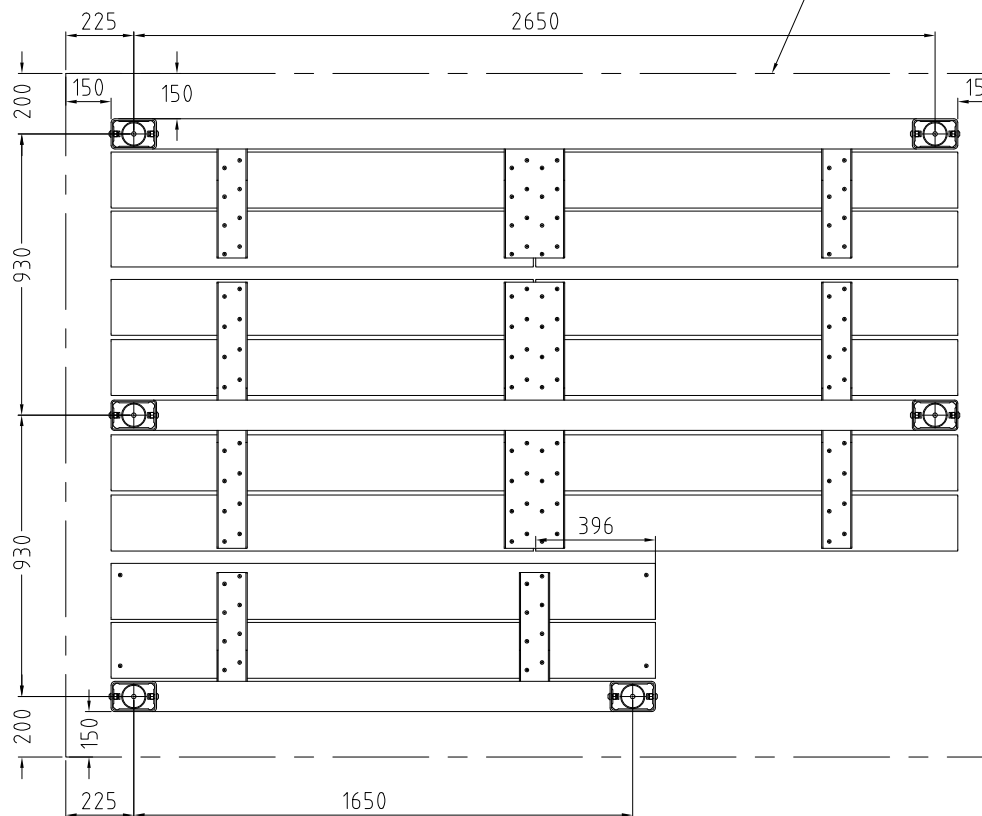
BOTTOM VIEW
