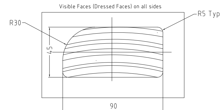
Timber Profile Front Slat
