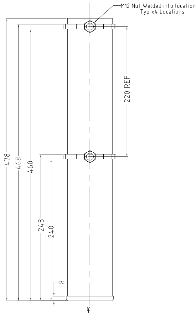
LEFT VIEW
