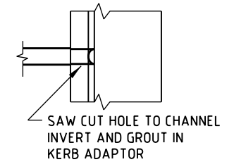
KERB ENTRY DETAIL
