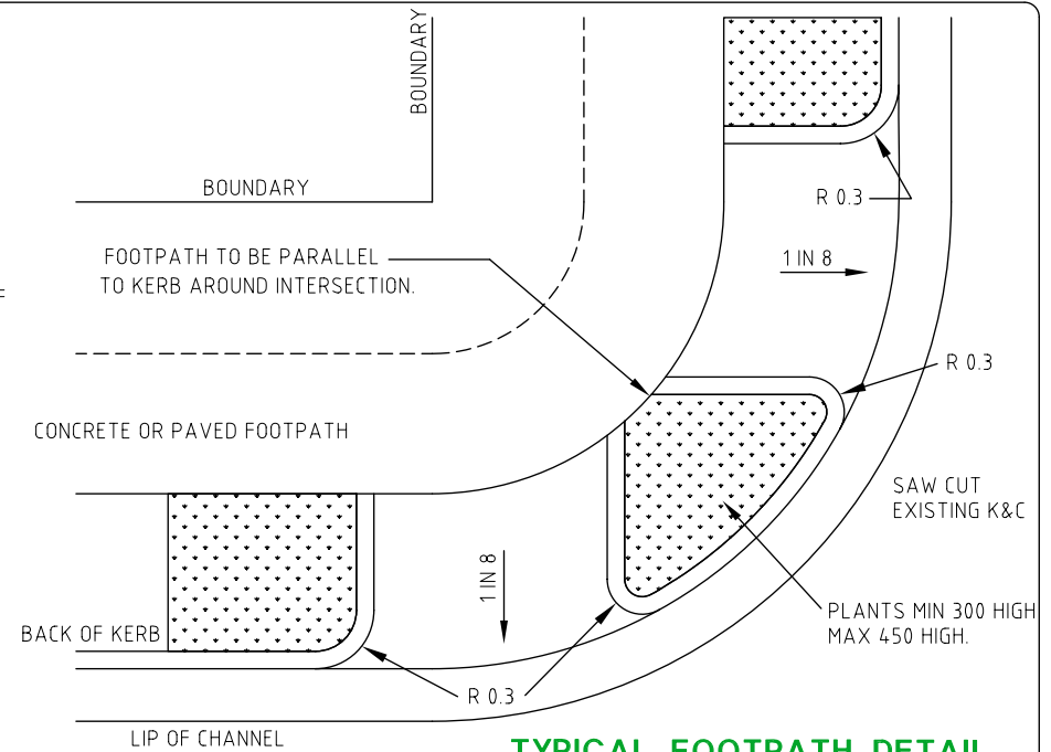
TYPICAL FOOTPATH DETAIL AT INTERSECTIONS
