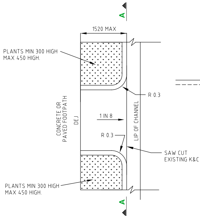
FOOTPATH KERB RAMP PLAN
