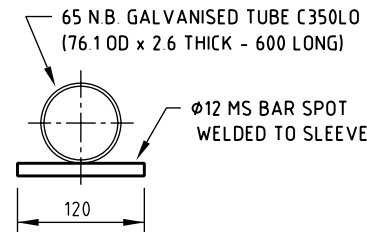
POST SLEEVE DETAIL
