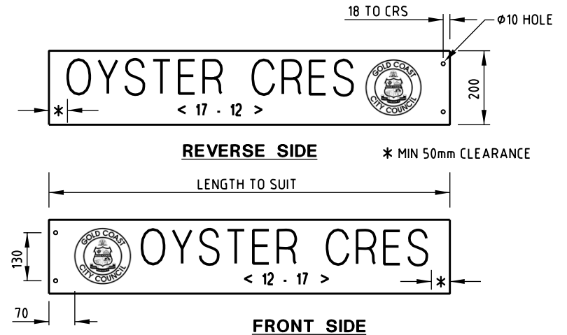
NAME PLATE
