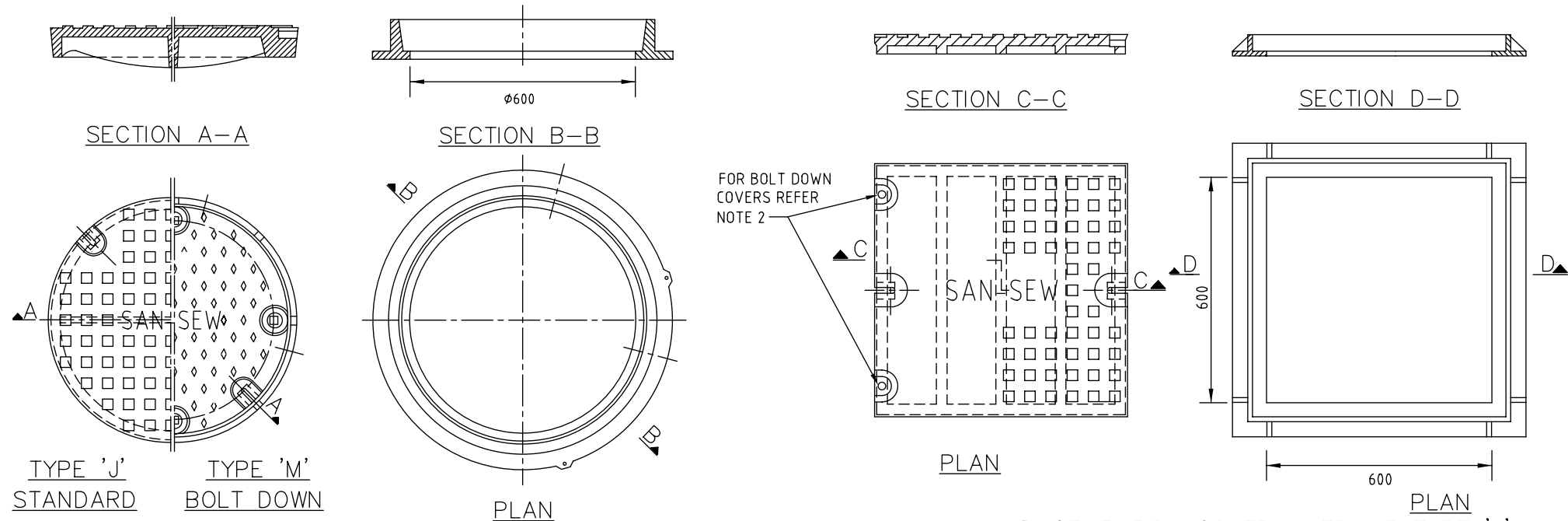
DUCTILE IRON COVER & FRAME TYPES 'J' AND 'M'
