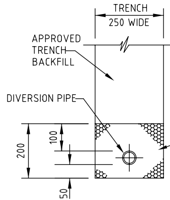
SECTION A-A DIVERSION DRAIN TRENCH
