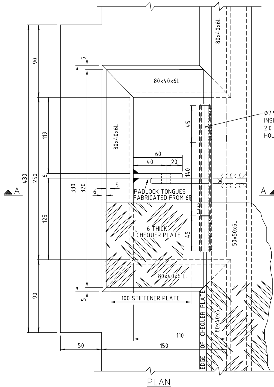
PADLOCK RECESS DETAIL
